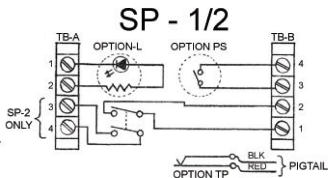
MODEL SP-1 (SINGLE POLE) MODEL SP-2 (DOUBLE POLE)
